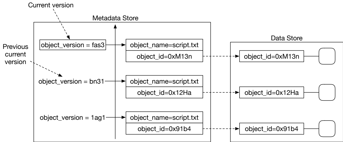
Figure 23 Versioned metadata
