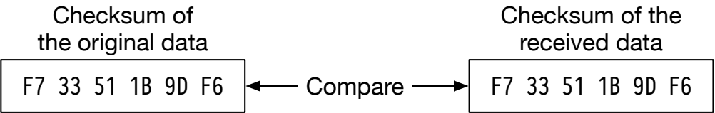
Figure 19 Compare checksums
