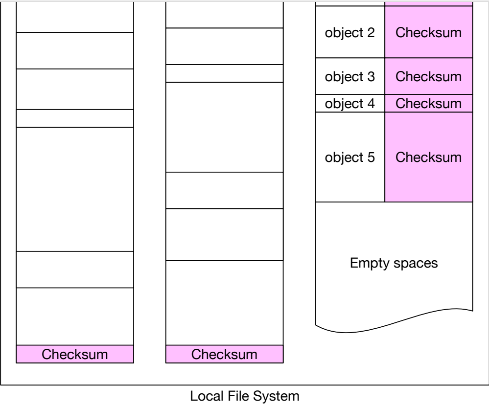
Figure 20 Add checksum to data node
