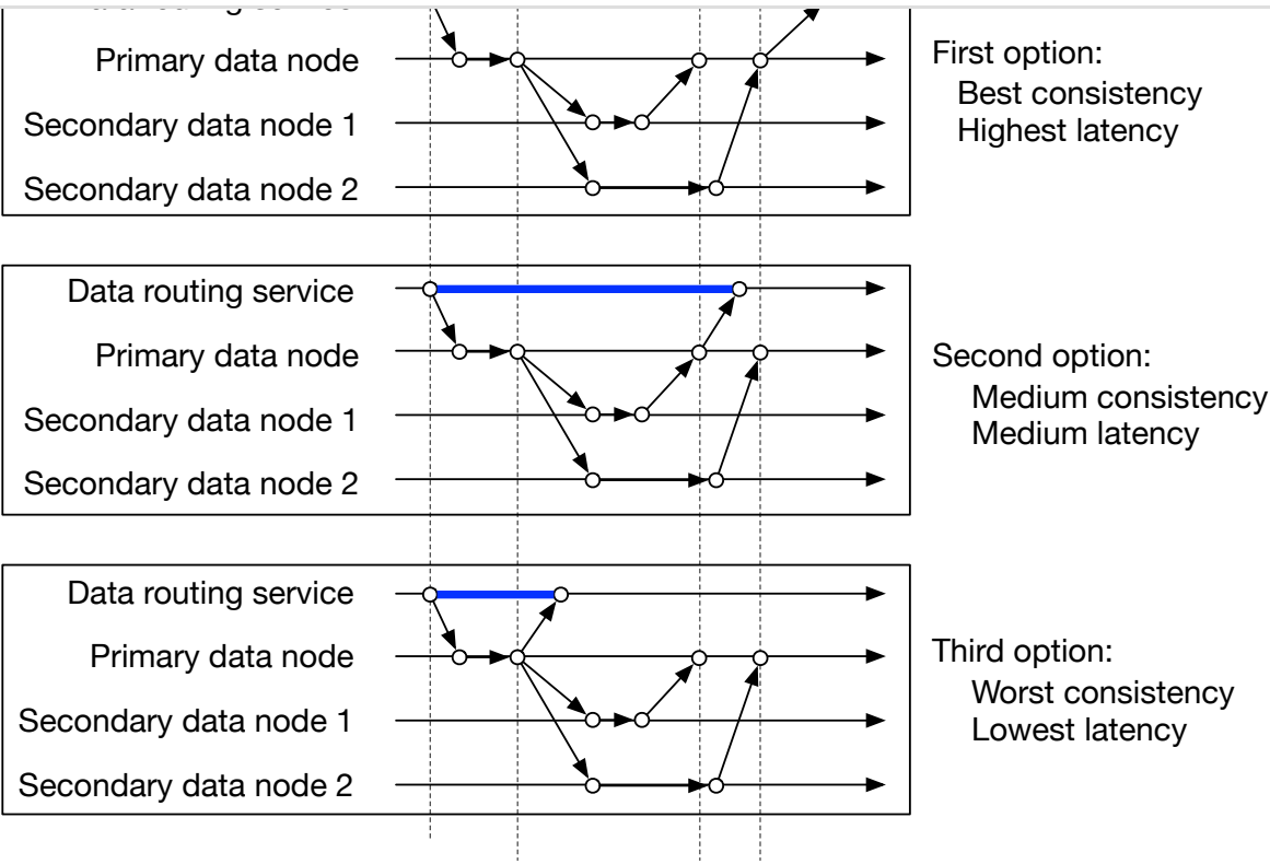
Figure 11 Trade-off between consistency and latency
