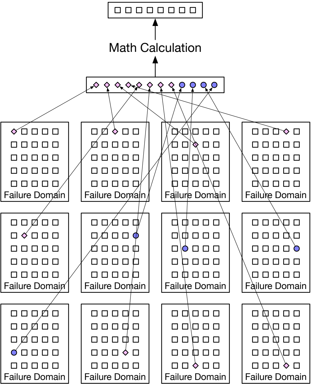
Figure 16 (8+4) erasure coding
