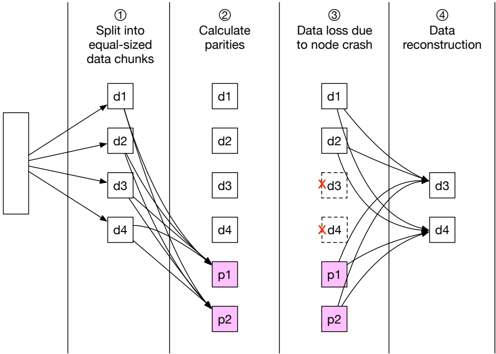
Figure 15 Erasure coding
