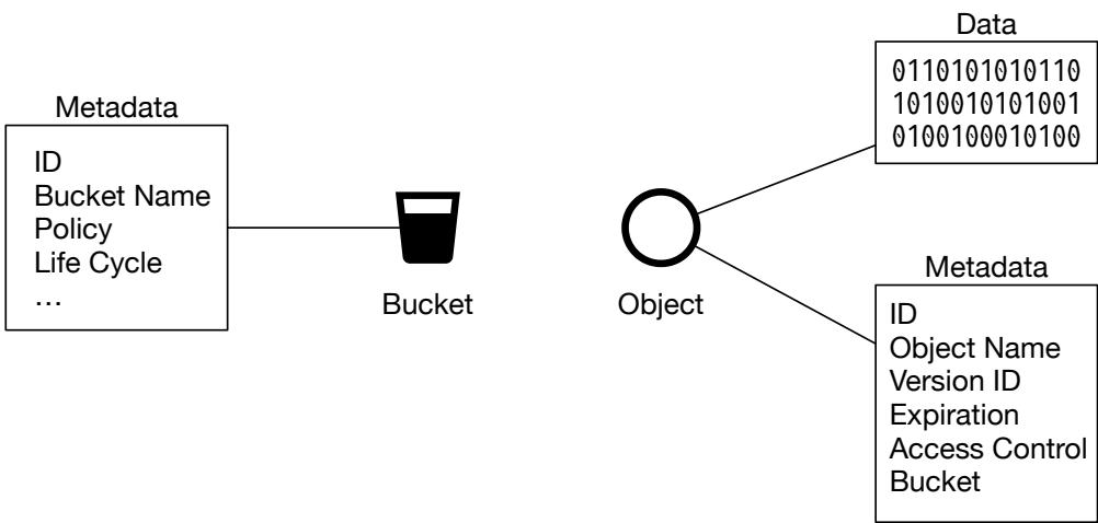
Figure 3 Bucket & object
