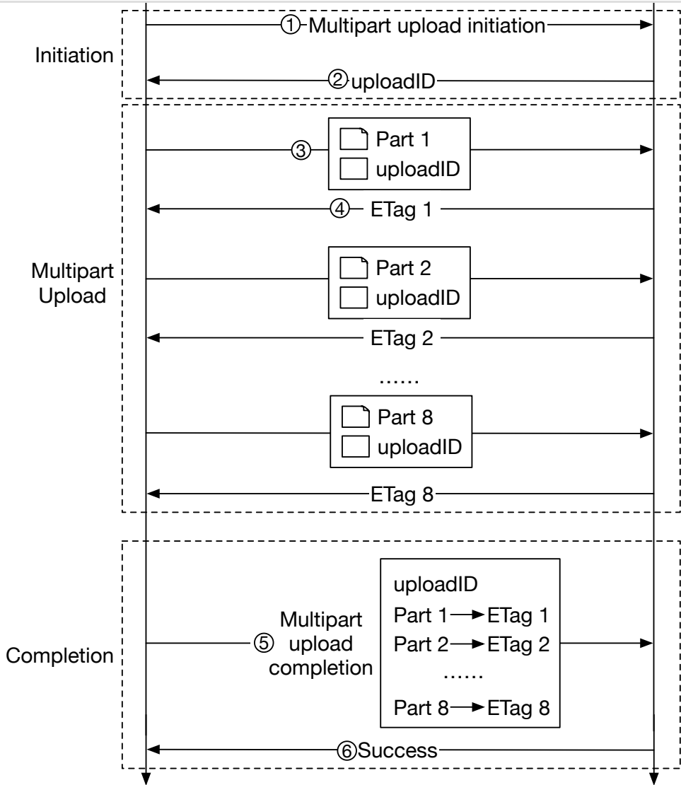
Figure 25 Multipart upload
