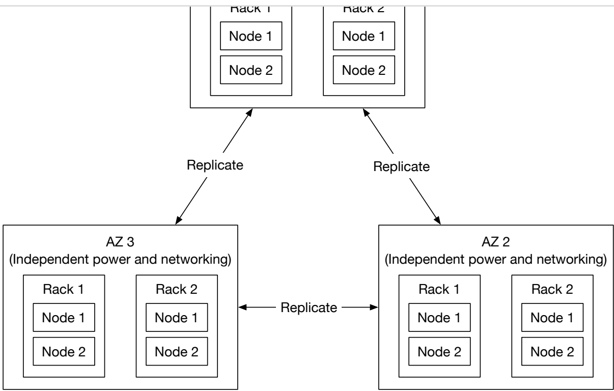
Figure 14 Multi-datacenter replication
