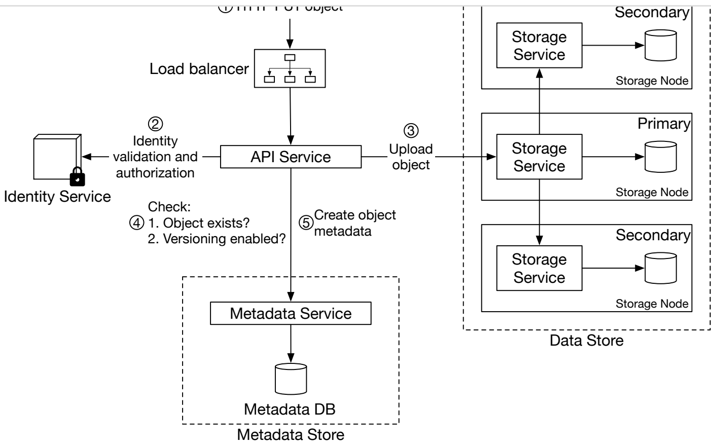
Figure 22 Object versioning
