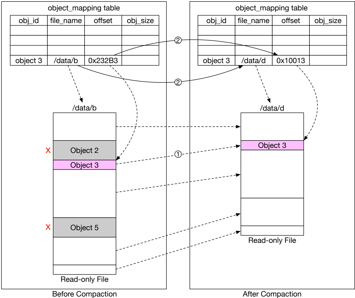
Figure 26 Compaction
