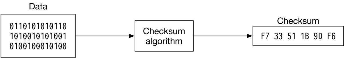
Figure 18 Generate checksum
